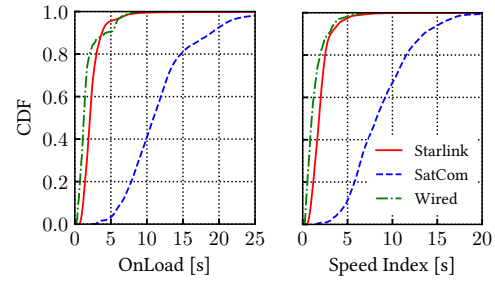
(a) onLoad.
